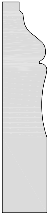
BA 3503LH 3/4 X 3-1/2
