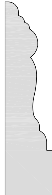
BA 3255LH 13/16 X 3-1/4
