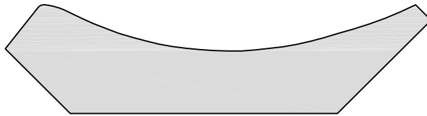
CO 3210 .820 X 3.210
