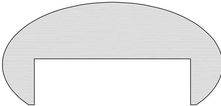
HR 3875 1-13/16 x 3-7/8
