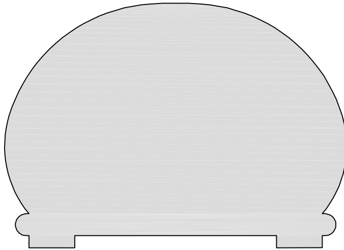
HR 3500 2-1/2 x 3-1/2
